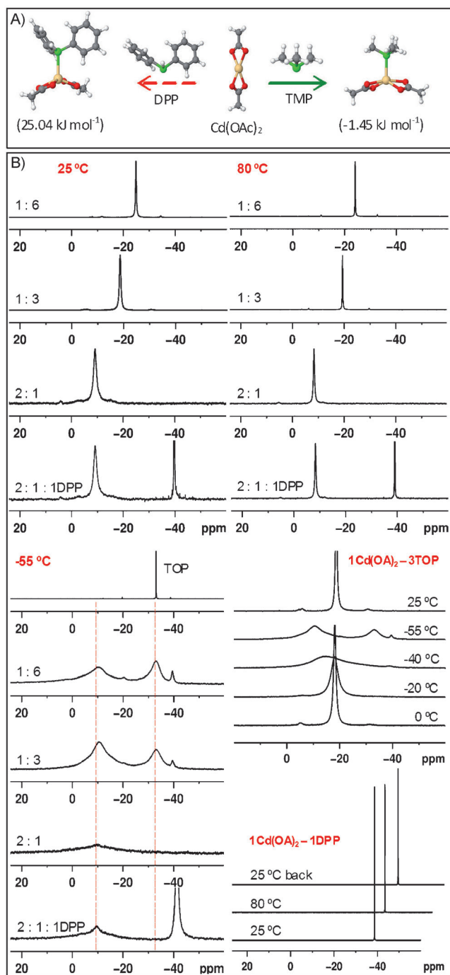
Figure 1. A) DFT calculations of the coordination between \text{Cd}(\text{OAc})_2 and TOP or DPP (Cd yellow; P green; C gray; H white; O red). The calculated changes in Gibbs free energy are shown in parentheses. B) In situ ^{31}\text{P} NMR spectra of the coordination from five mixtures of \text{Cd}(\text{OAc})_2 (X) and TOP (Y) and/or DPP (Z) with the different feed molar ratios (in the form X:Y:Z) and at the temperatures indicated. Also, the ^{31}\text{P} NMR spectra of TOP at -55^\circ\text{C} is shown.
